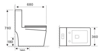
T2130MG WASHDOWN ONE-PIECE TOILET Size: 680x360x780mm S-trap : 250mm Roughing-in P-trap : 180mm Roughing-in
