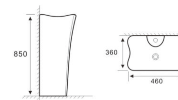
P3202MG STANDING BASIN Size: 460x360x850mm Installation: Fixing to wall with back
