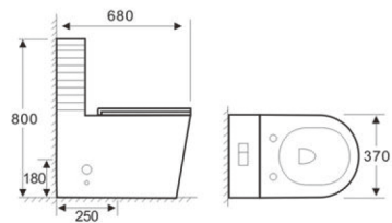
T2126 WASHDOWN ONE-PIECE TOILET Size: 680x370x800mm S-trap : 250mm Roughing-in P-trap : 180mm Roughing-in
