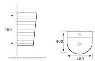
P126 WALL-HUNG BASIN Size: 400x400x450mm Wall-hung Installation
