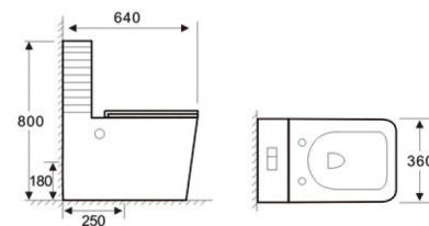
T2079 WASHDOWN ONE-PIECE TOILET Size: 640x360x800mm S-trap : 250mm Roughing-in P-trap : 180mm Roughing-in
