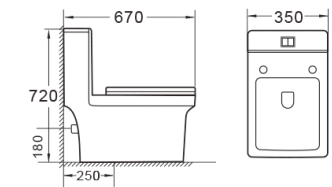
T2071 WASHDOWN ONE-PIECE TOILET Size: 670x350x720mm S-trap: 250mm Roughing-in P-trap: 180mm Roughing-in
