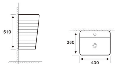
P179 WALL-HUNG BASIN Size: 400x380x510mm Wall-hung Installation
