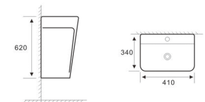
P130MG WALL-HUNG BASIN Size: 410x340x620mm Wall-hung Installation
