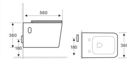
T3201 WALL-HUNG TOILET Size: 560x360x360mm Washdown/P-trap P-trap: 180mm Roughing-in
